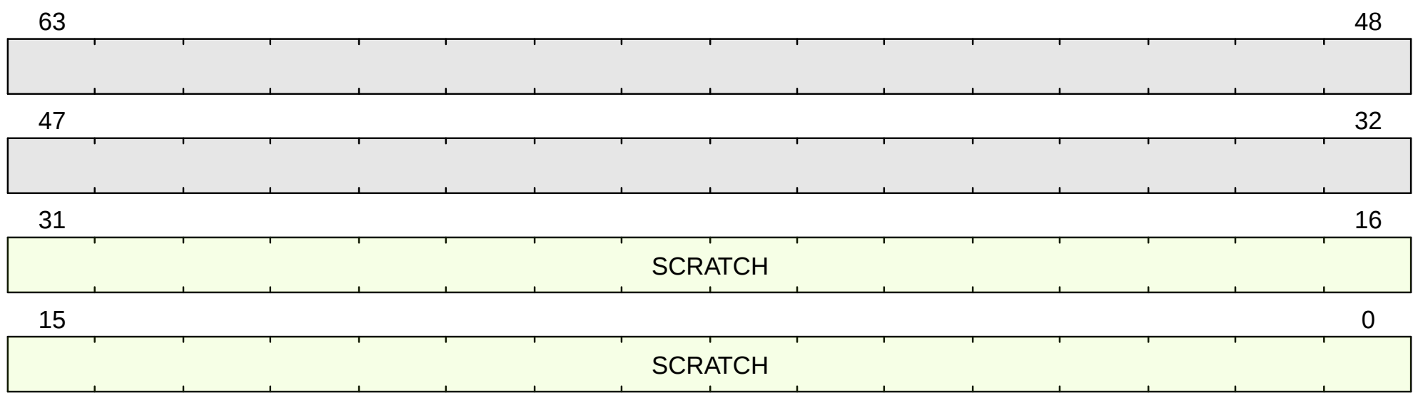
Figure 14. mscratch format
