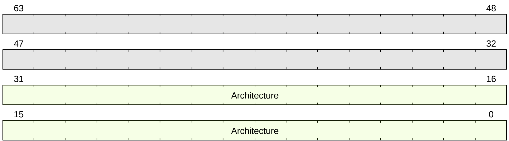
Figure 3. marchid format
