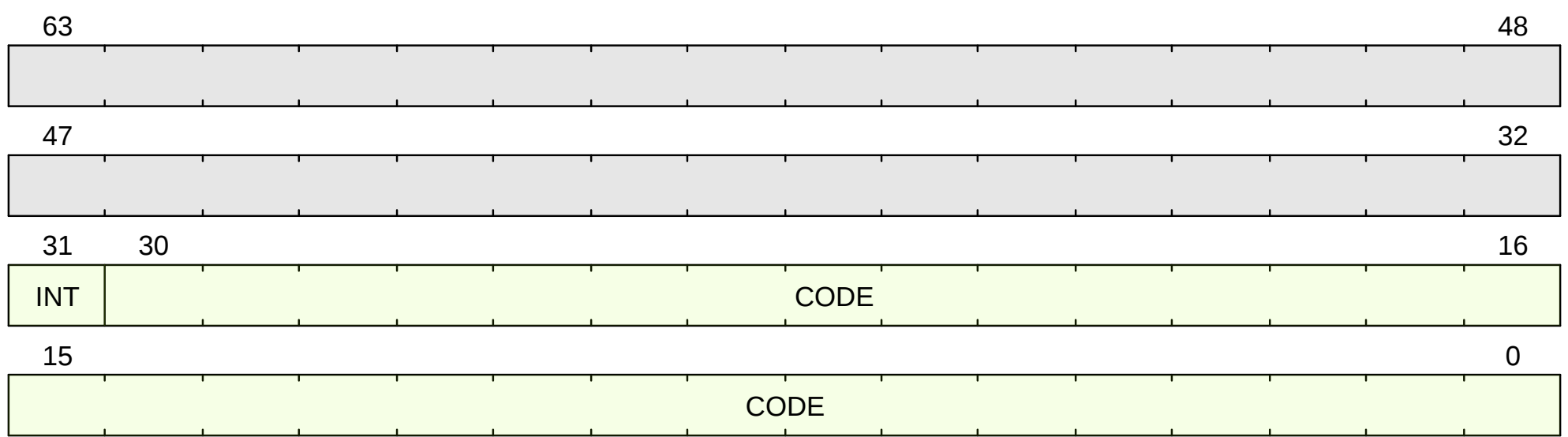
Figure 4. mcause format
