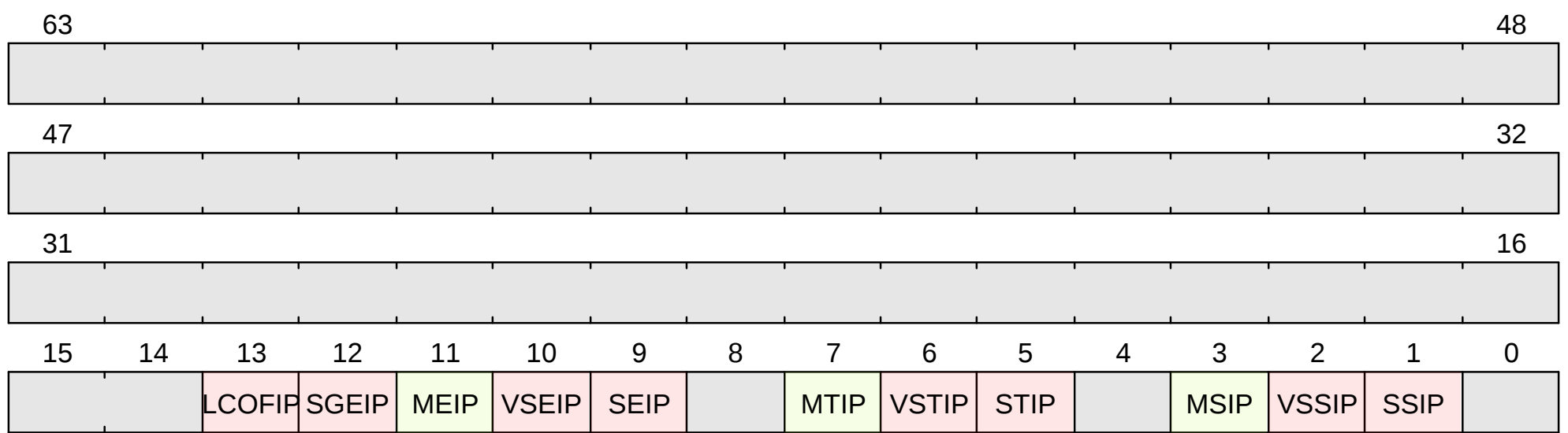
Figure 12. mip format
