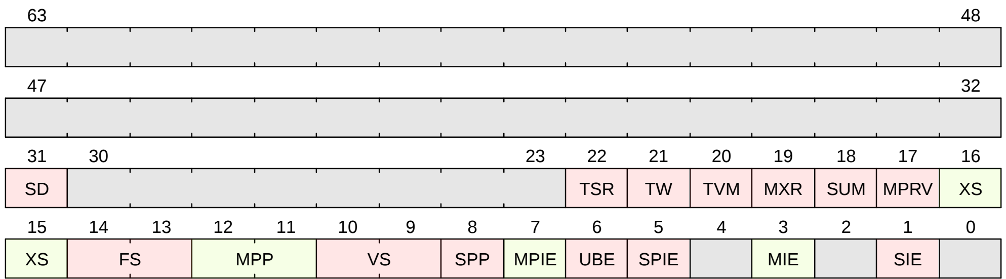
Figure 15. mstatus format
