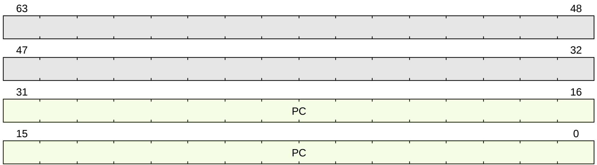
Figure 7. mepc format
