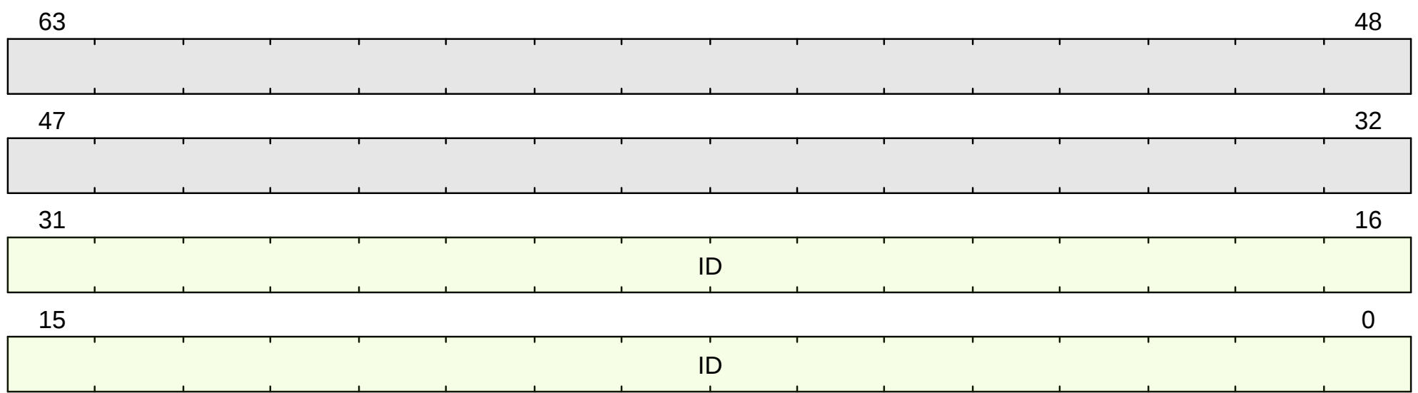
Figure 8. mhartid format
