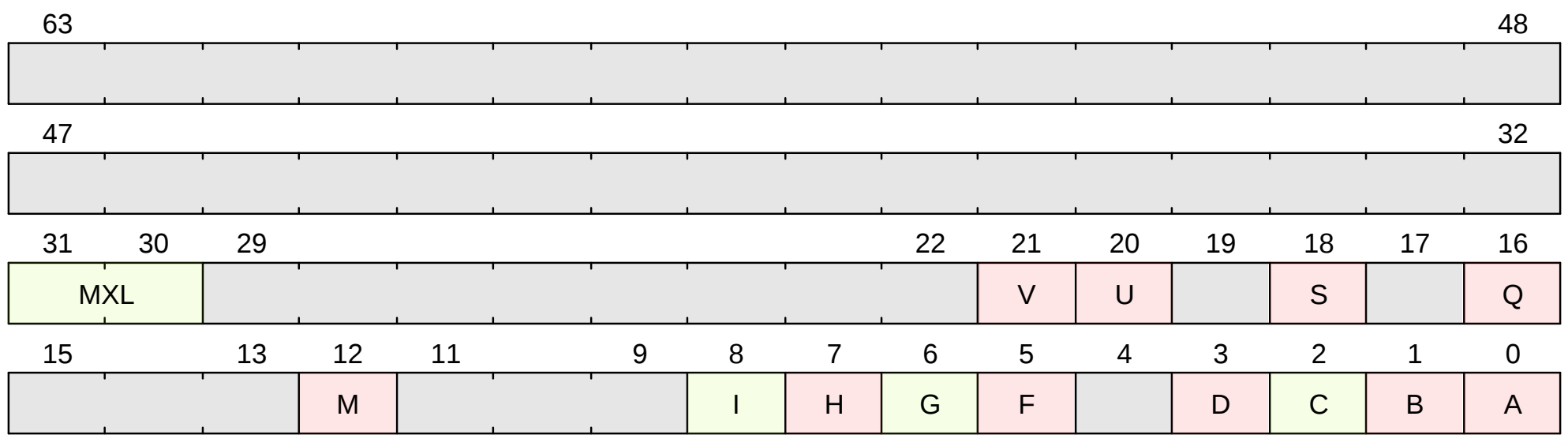
Figure 13. misa format
