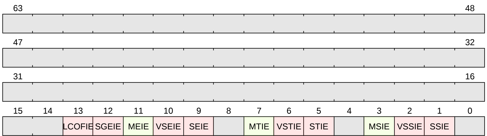
Figure 9. mie format
