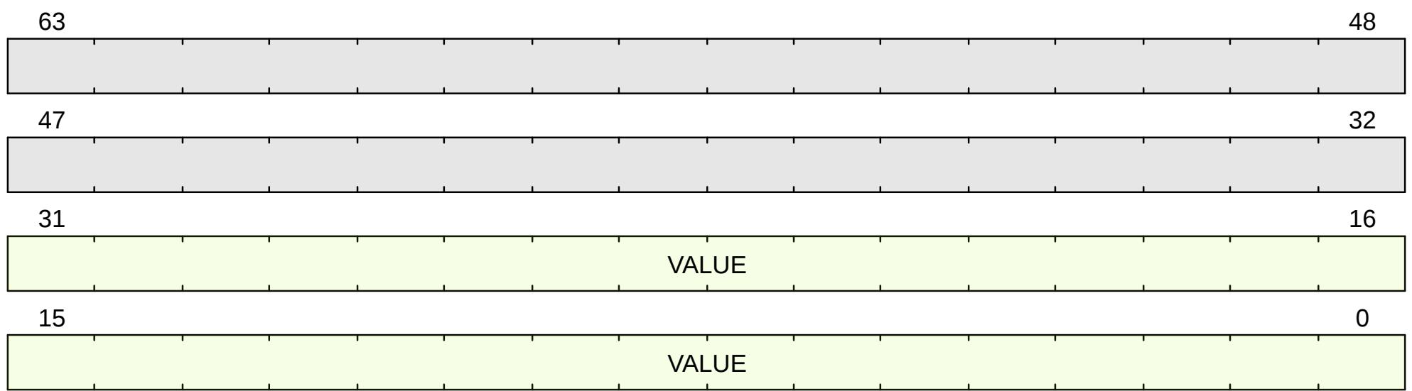
Figure 16. mtval format
