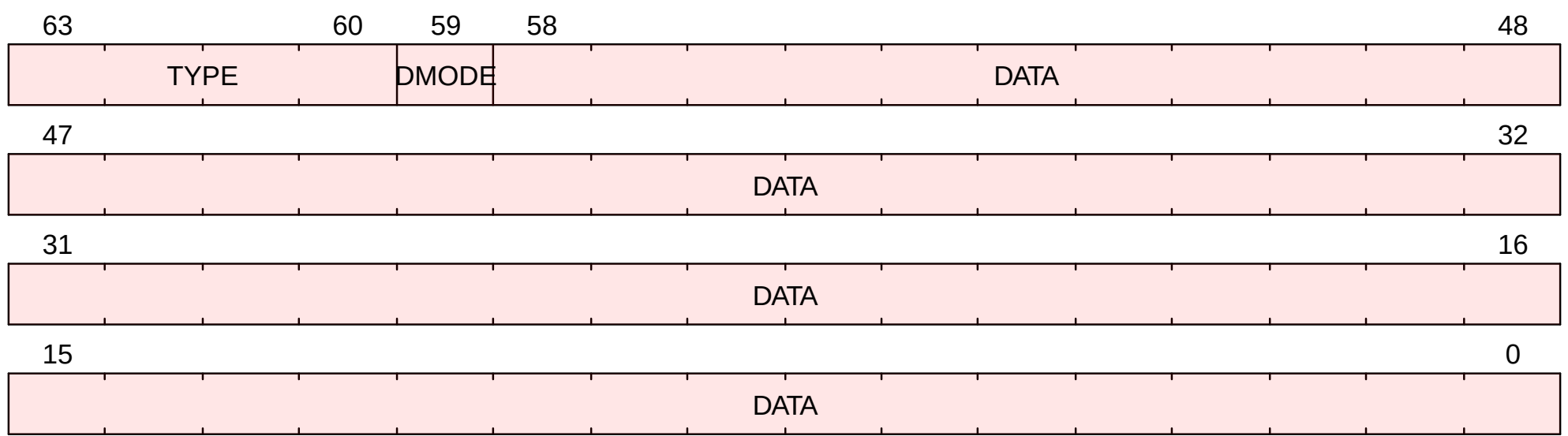
Figure 52. tdata1 Format when (priv_mode() == PrivilegeMode::M && CSR[misa].MXL == 1) || (priv_mode() == PrivilegeMode::S && CSR[mstatus].SXL == 1) || (priv_mode() == PrivilegeMode::VS && CSR[hstatus].VSXL == 1)
