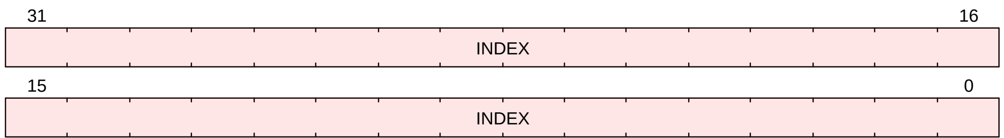
Figure 58. tselect Format when (priv_mode() == PrivilegeMode::M && CSR[misa].MXL == 0) || (priv_mode() == PrivilegeMode::S && CSR[mstatus].SXL == 0) || (priv_mode() == PrivilegeMode::VS && CSR[hstatus].VSXL == 0)
