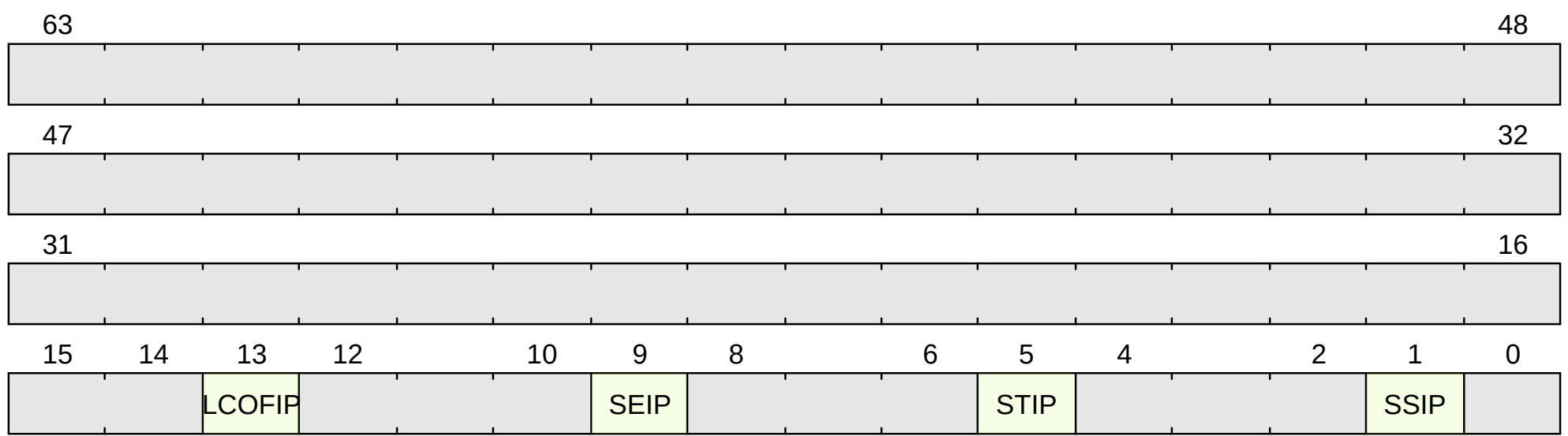
Figure 45. sip format
