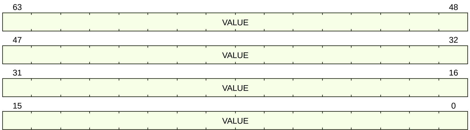
Figure 49. stval format
