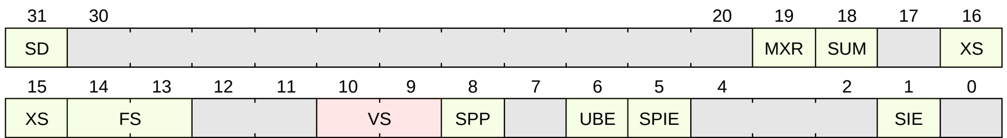
Figure 47. sstatus Format when CSR[mstatus].SXL == 0
