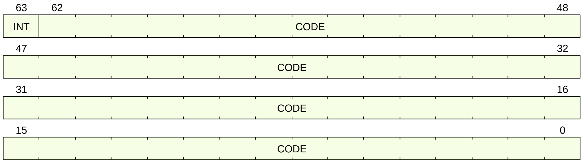
Figure 41. scause Format when CSR[mstatus].SXL == 1
