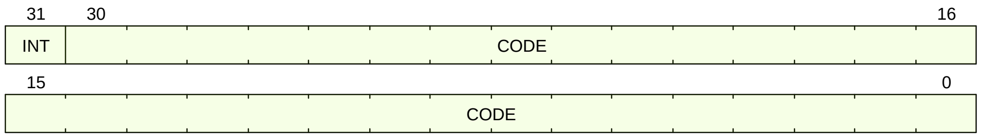
Figure 40. scause Format when CSR[mstatus].SXL == 0
