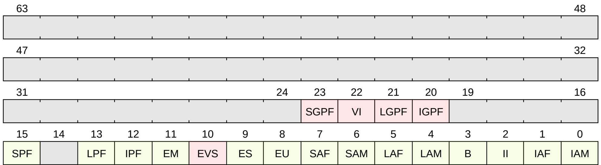
Figure 37. medeleg format
