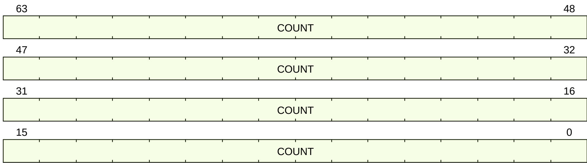
Figure 22. hpmcounter27 format
