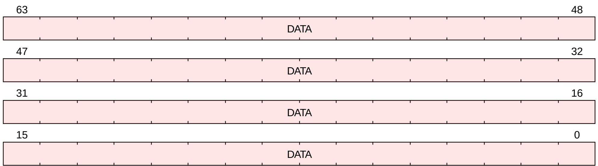
Figure 54. tdata2 Format when (priv_mode() == PrivilegeMode::M && CSR[misa].MXL == 1) || (priv_mode() == PrivilegeMode::S && CSR[mstatus].SXL == 1) || (priv_mode() == PrivilegeMode::VS && CSR[hstatus].VSXL == 1)
