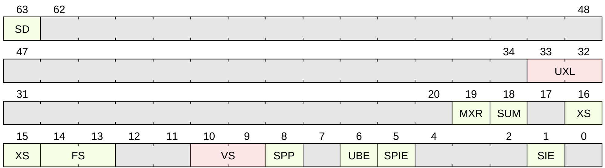
Figure 48. sstatus Format when CSR[mstatus].SXL == 1
