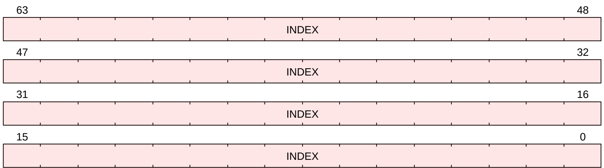
Figure 59. tselect Format when (priv_mode() == PrivilegeMode::M && CSR[misa].MXL == 1) || (priv_mode() == PrivilegeMode::S && CSR[mstatus].SXL == 1) || (priv_mode() == PrivilegeMode::VS && CSR[hstatus].VSXL == 1)
