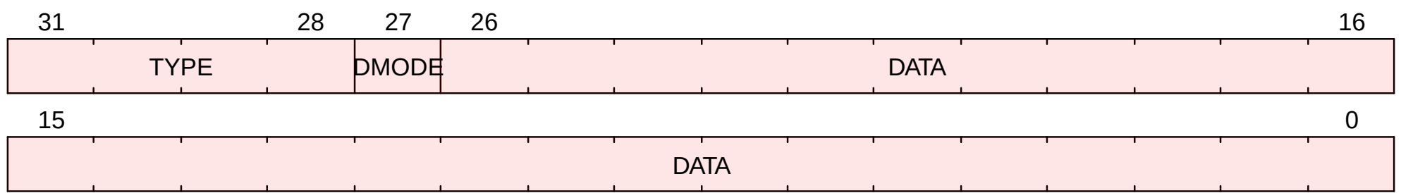
Figure 51. tdata1 Format when (priv_mode() == PrivilegeMode::M && CSR[misa].MXL == 0) || (priv_mode() == PrivilegeMode::S && CSR[mstatus].SXL == 0) || (priv_mode() == PrivilegeMode::VS && CSR[hstatus].VSXL == 0)
