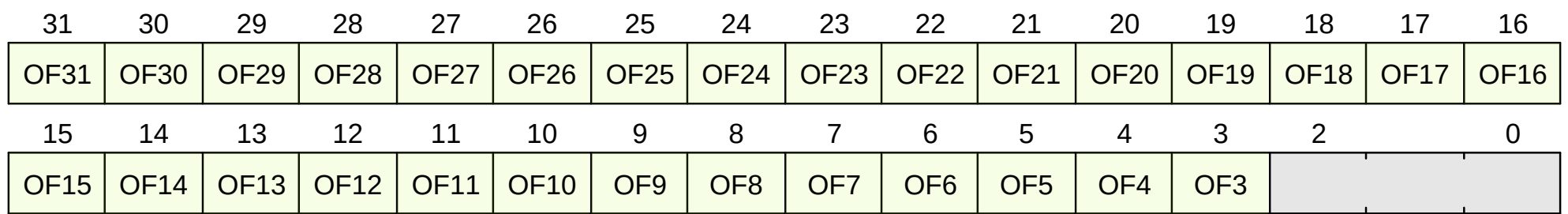
Figure 43. scountovf format
