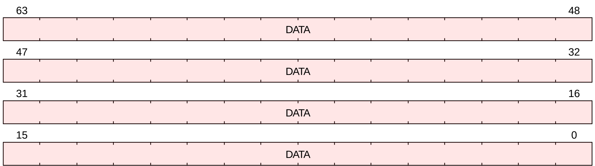
Figure 56. tdata3 Format when (priv_mode() == PrivilegeMode::M && CSR[misa].MXL == 1) || (priv_mode() == PrivilegeMode::S && CSR[mstatus].SXL == 1) || (priv_mode() == PrivilegeMode::VS && CSR[hstatus].VSXL == 1)
