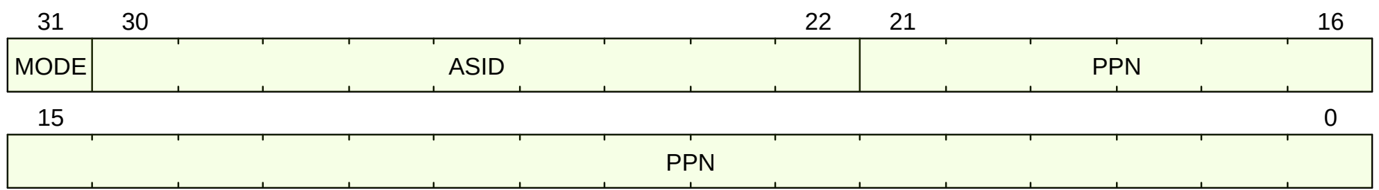
Figure 38. satp Format when CSR[mstatus].SXL == 0
