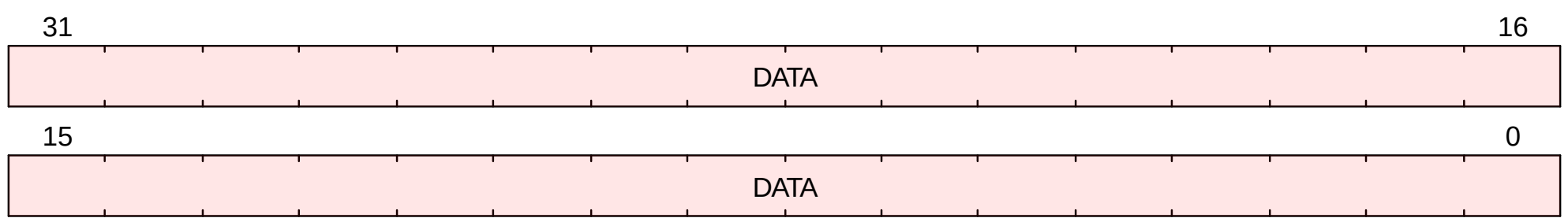
Figure 55. tdata3 Format when (priv_mode() == PrivilegeMode::M && CSR[misa].MXL == 0) || (priv_mode() == PrivilegeMode::S && CSR[mstatus].SXL == 0) || (priv_mode() == PrivilegeMode::VS && CSR[hstatus].VSXL == 0)
