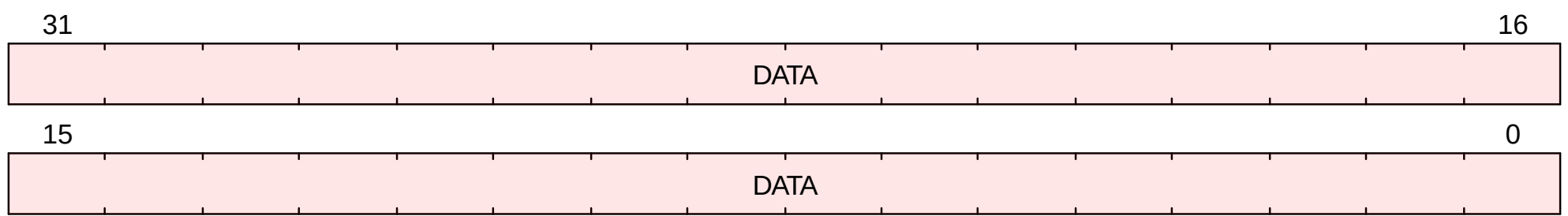
Figure 53. tdata2 Format when (priv_mode() == PrivilegeMode::M && CSR[misa].MXL == 0) || (priv_mode() == PrivilegeMode::S && CSR[mstatus].SXL == 0) || (priv_mode() == PrivilegeMode::VS && CSR[hstatus].VSXL == 0)
