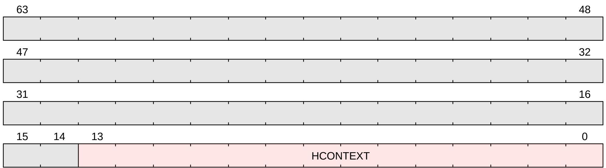
Figure 35. mcontext format
