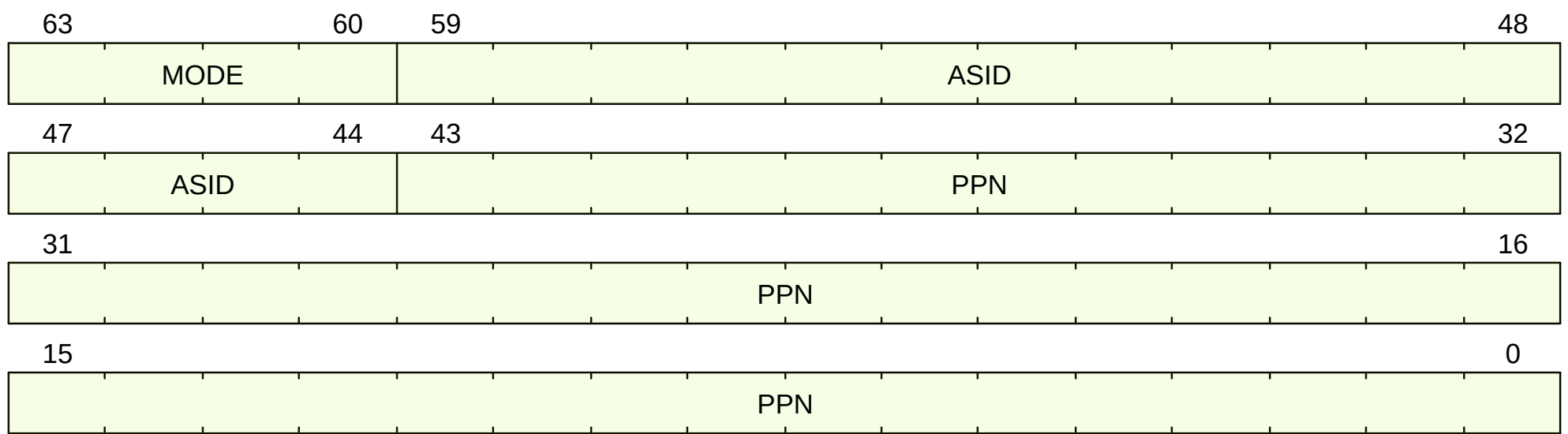
Figure 39. satp Format when CSR[mstatus].SXL == 1
