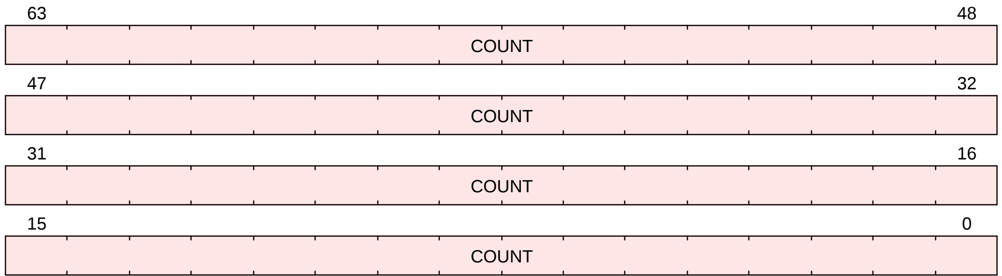
Figure 33. hpmcounter9 format
